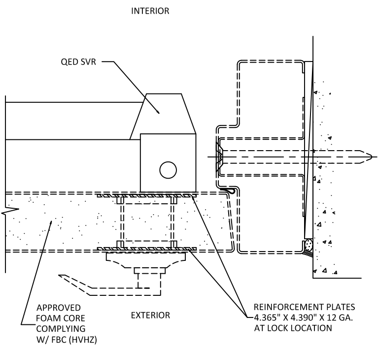
F 2 HORIZONTAL SECTION QED100 SVR SINGLE DOOR
